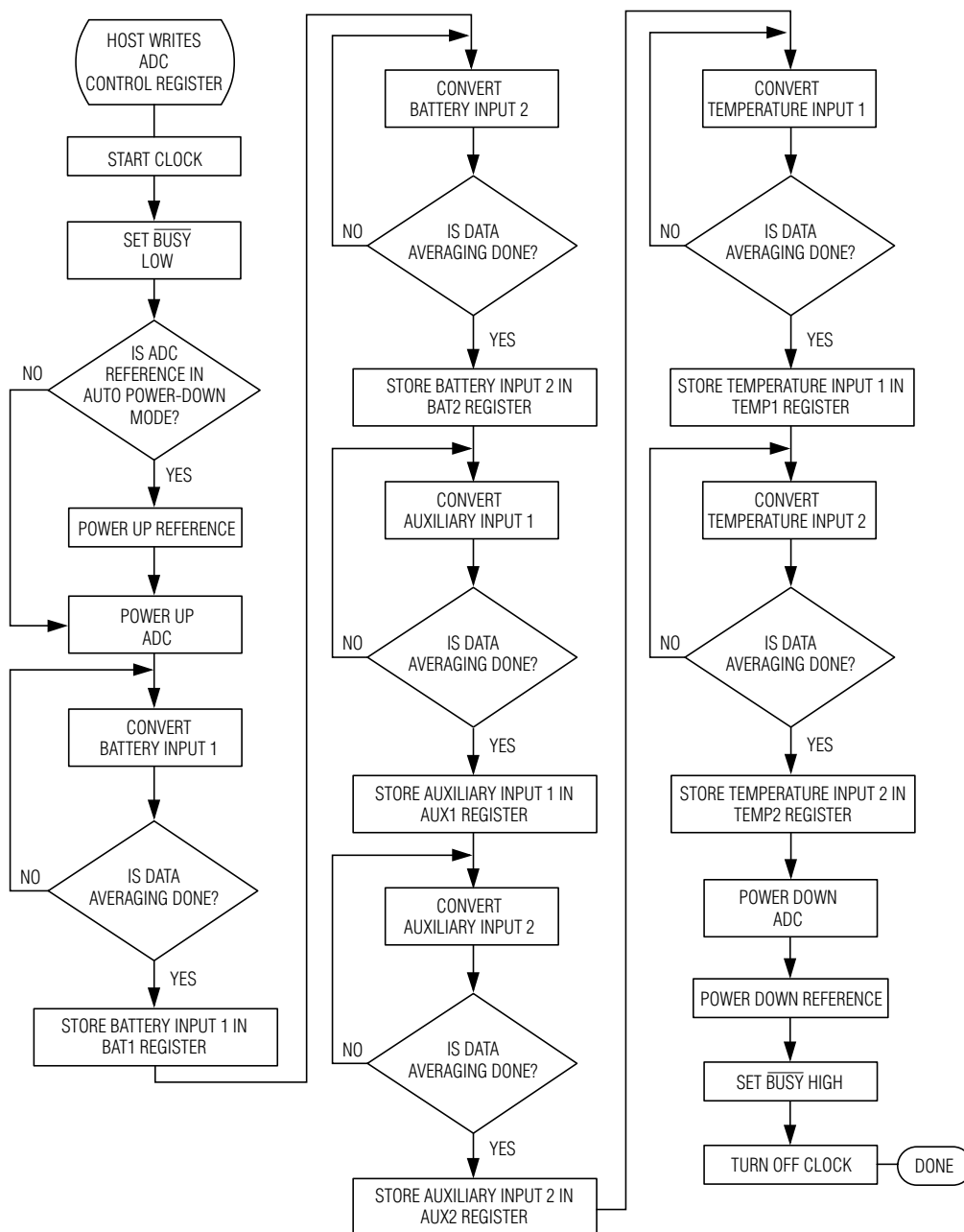
Figure 20. Scan Mode Flowchart
