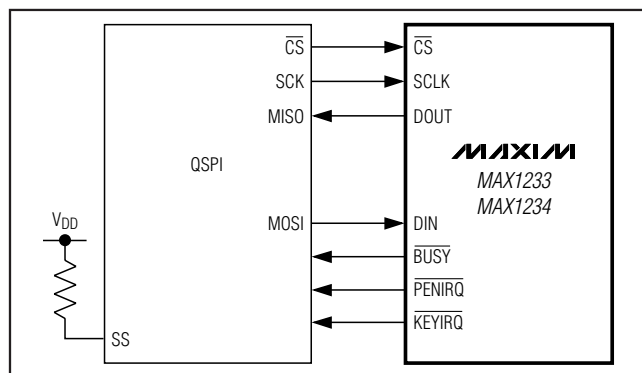
Figure 29. QSPI Interface
